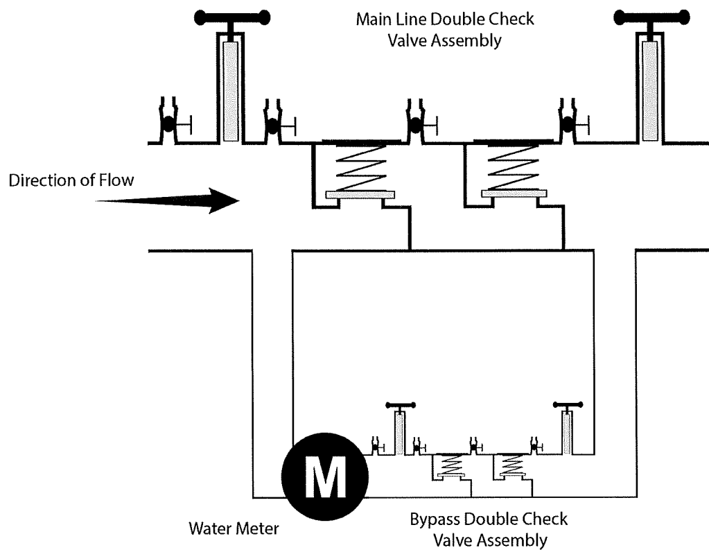
Diagram 1 Double check detector backflow prevention assembly 1
